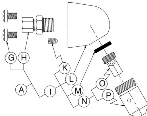
PENAL SHOWER HEAD FOR AIR-CONTROL VALVE #99150081
