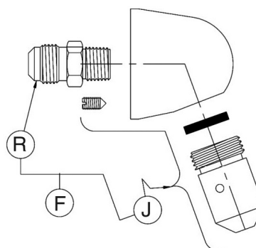
-SSV PENAL SHOWER HEAD FOR PENAL-TROL VALVE #99150082
