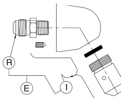
PENAL SHOWER HEAD FOR PENAL-TROL VALVE #99150080
